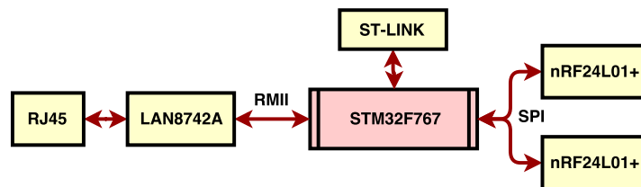
Fig. 8. Base Station Hardware Components
