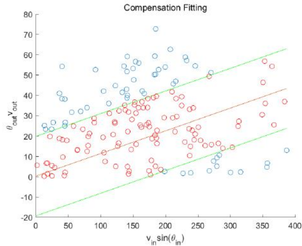
Fig. 16. Compensation Angle Fitting Using RANSAC
