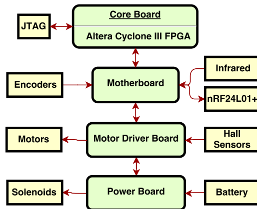
Fig. 5. Electrical System
