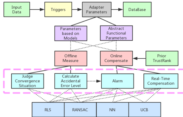
Fig. 14. Parameters Self-Adaption Flow Chart
