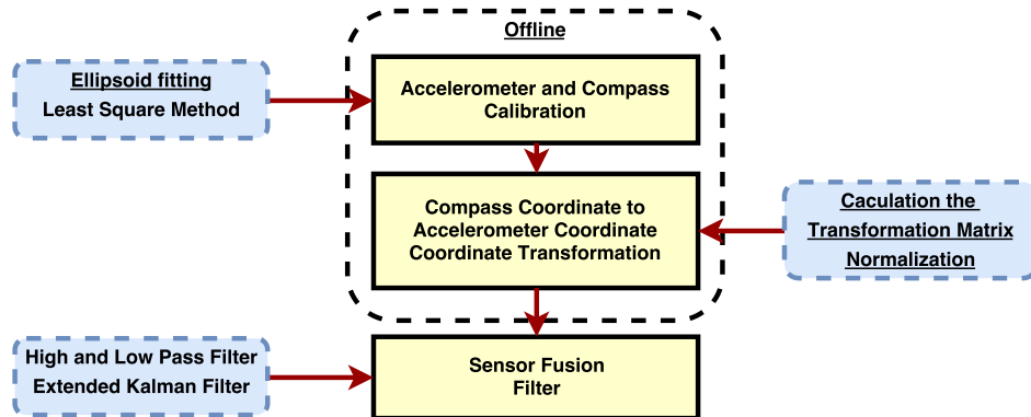
Fig. 7. Procedures of Sensor Fusion
