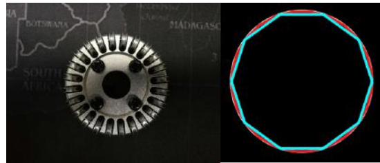
Fig. 1. Omni-directional Wheel and Polygon-Effect
