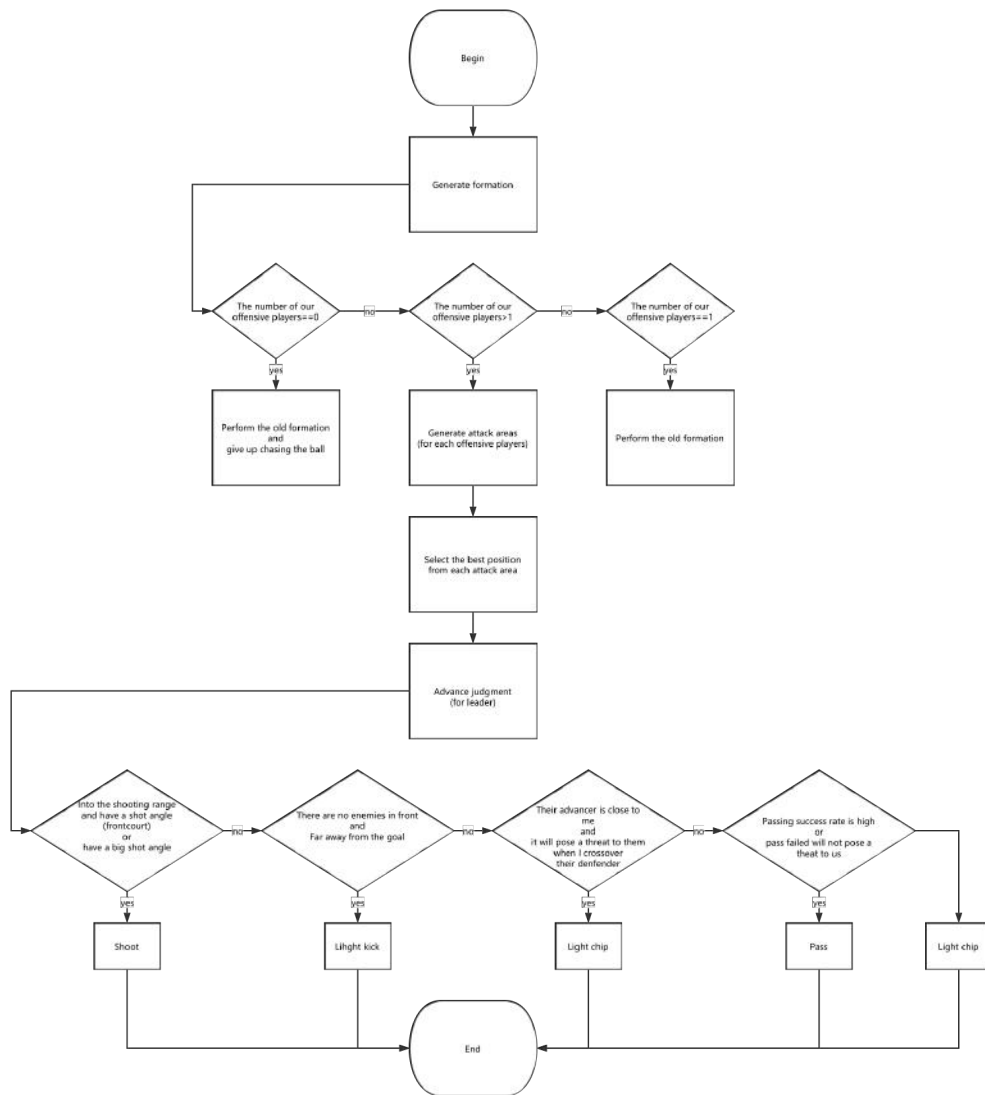
Fig. 18. Flow Chart of Decision Module
