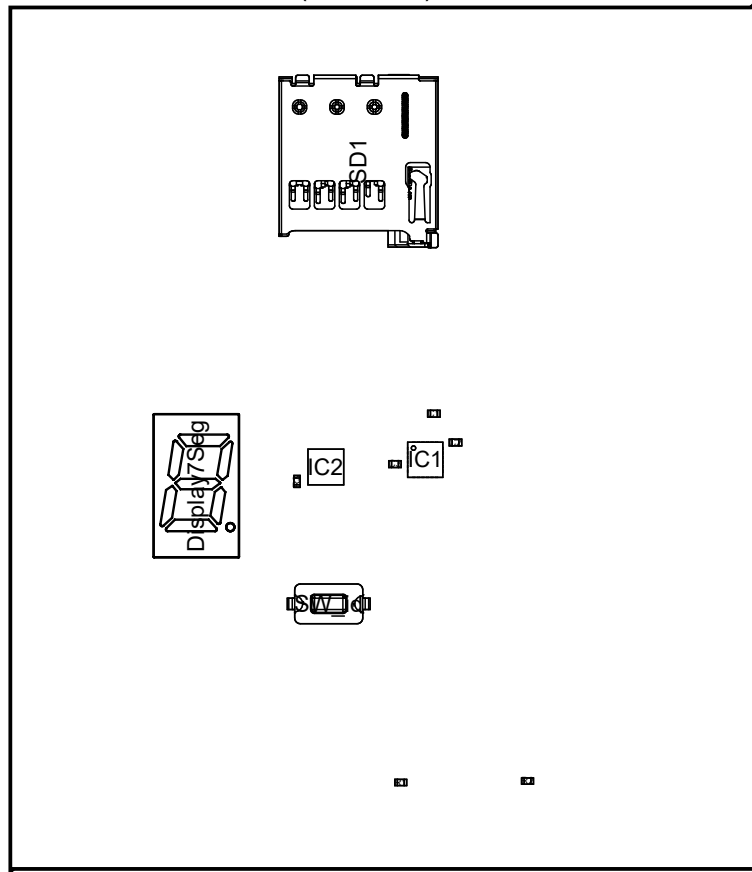
View from Bottom side (Scale 3:2)
